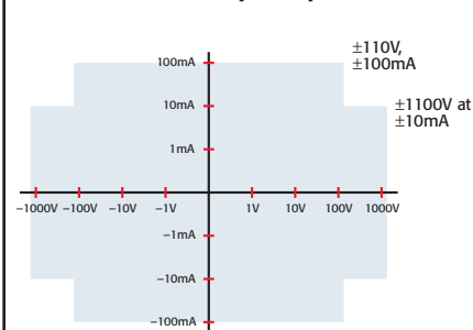
Model 237 Source Capability
