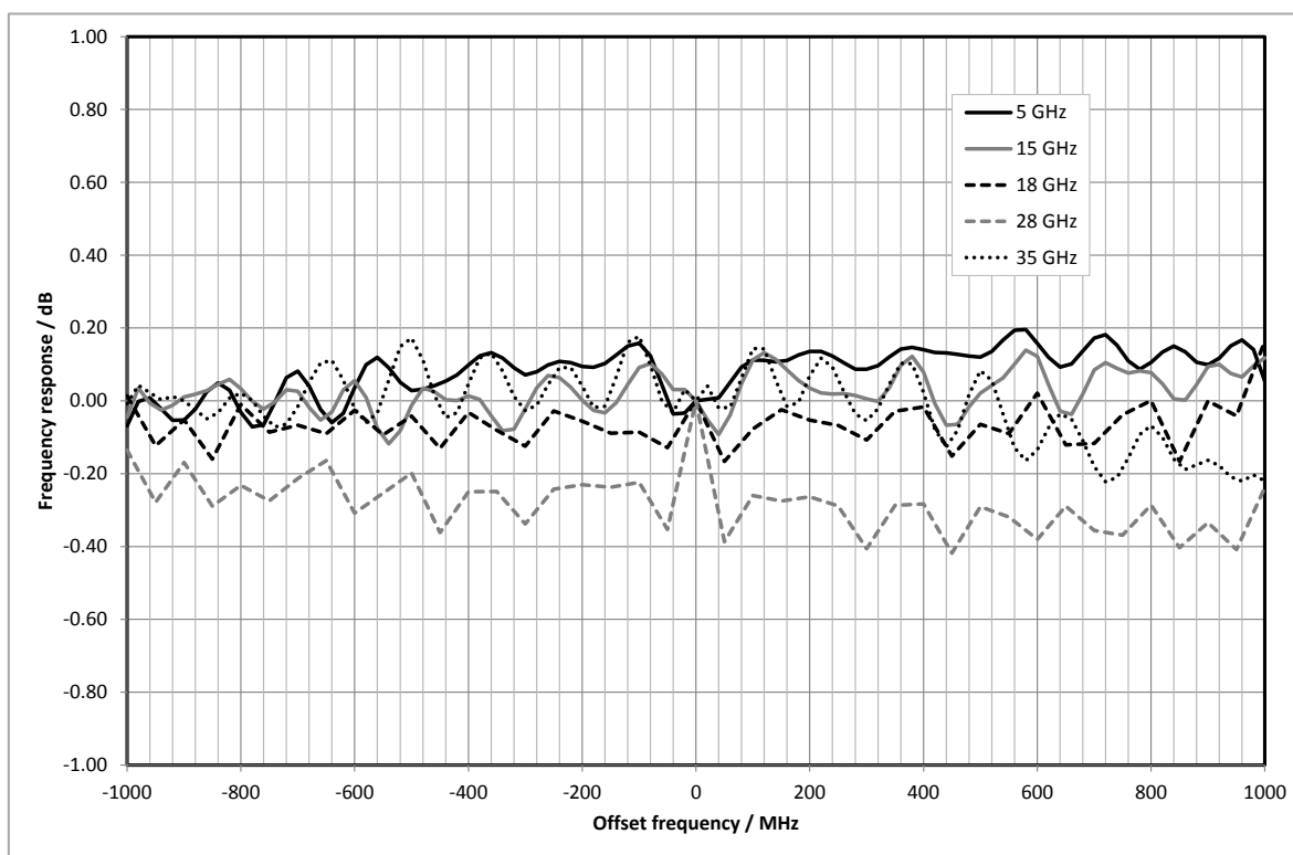
Measured RF modulation frequency response with internal baseband I/Q, wideband baseband
