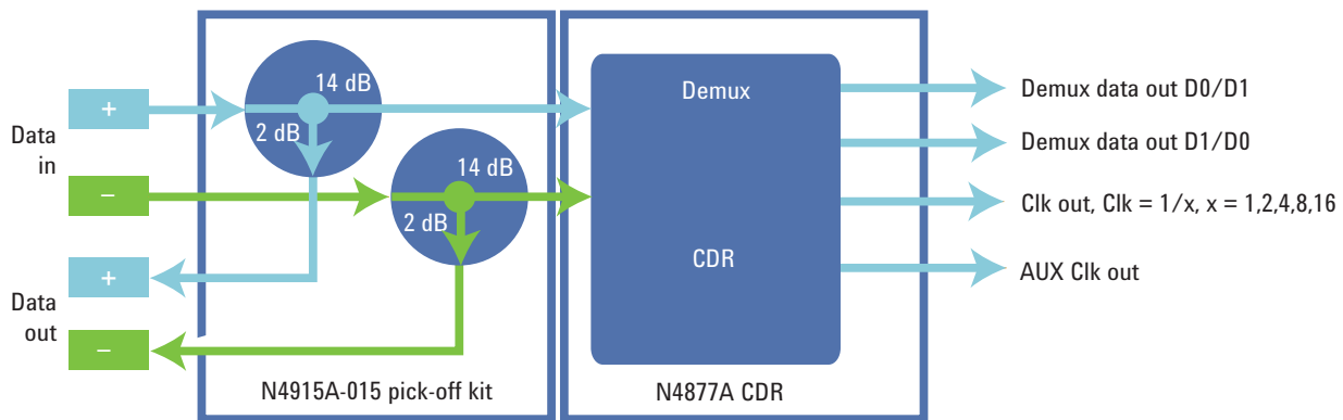
Figure 3. The N4915A-015 pick-off kit is especially designed to be used with the N4877A and offers a bandwidth of 50 GHz. The demultiplexer data outputs can swap between even and odd bits.
