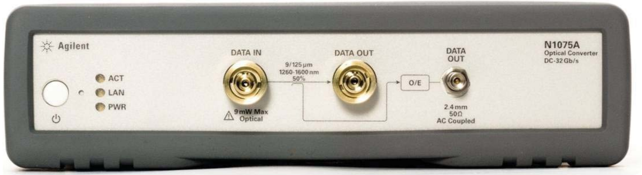
Figure 14. A front panel view of the Agilent N1075A M14 optical pick-off/converter.
