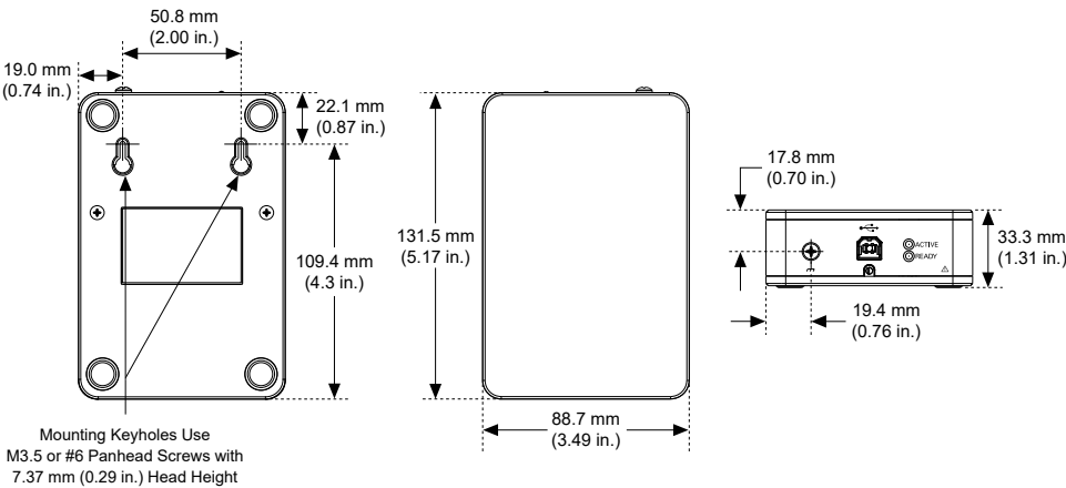
Figure 1. cDAQ-9171 Dimensions
