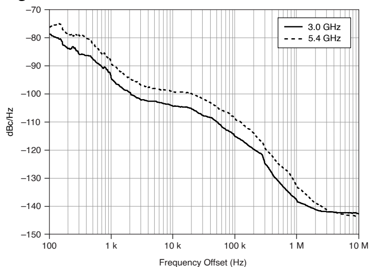
Figure 4. Measured Phase Noise at 3.0 GHz in Narrow and Wide Loop Bandwidth (0 dBm Output)
