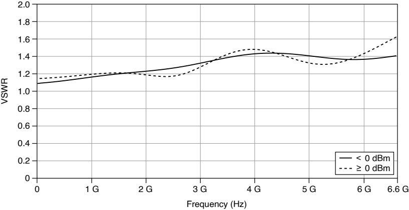
Figure 1. Measured VSWR
