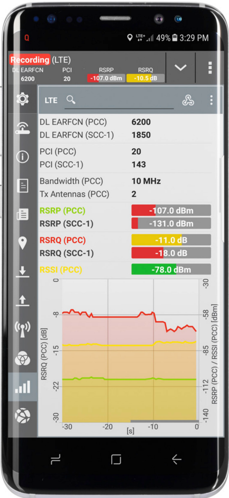
The Android based QualiPoc application running on a smartphone controls the R&S®TSMA6.
