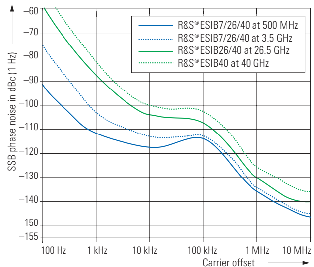
Typical SSB phase noise
